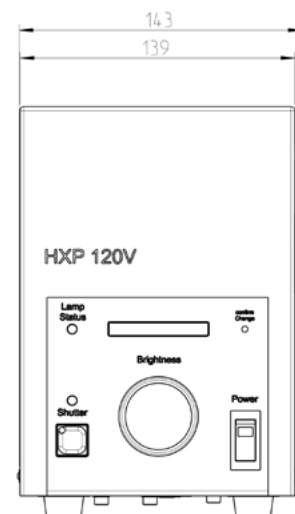
Front view of LQ-HXP 120 | Dimensions in mm
