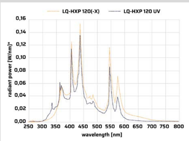
Spectrum HXP 120(-X) and HXP 120 UV
